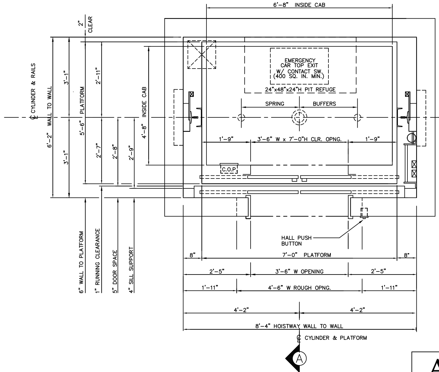
HOISTWAY PLAN
