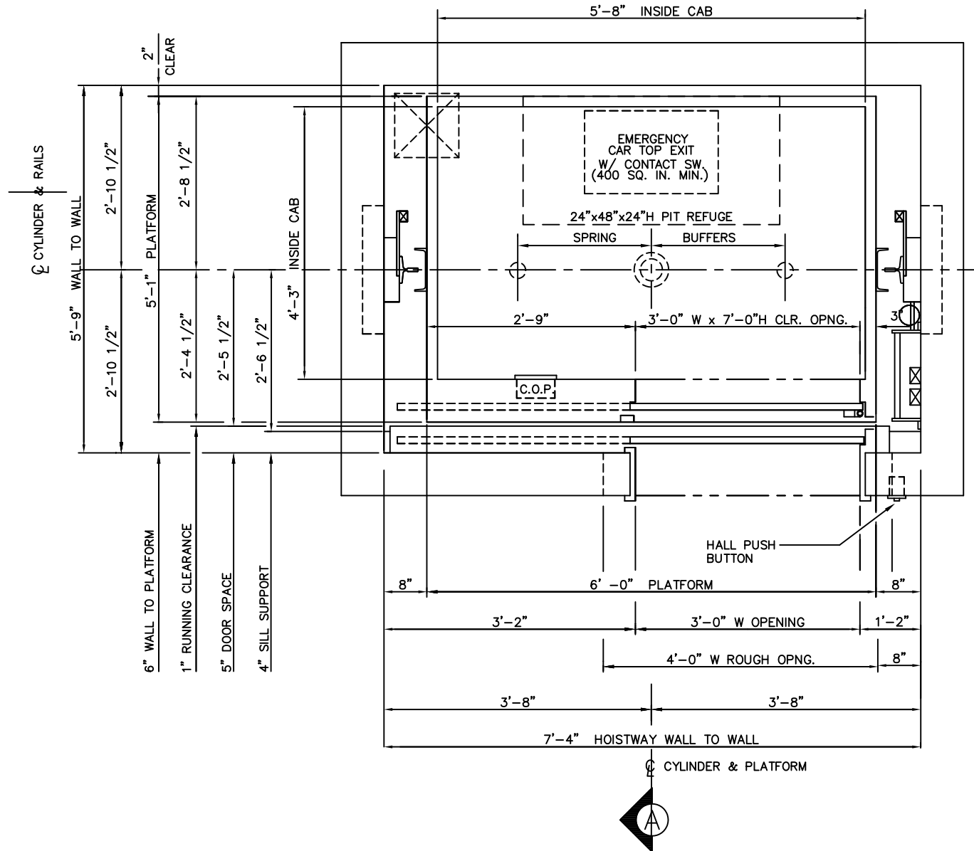
HOISTWAY PLAN
