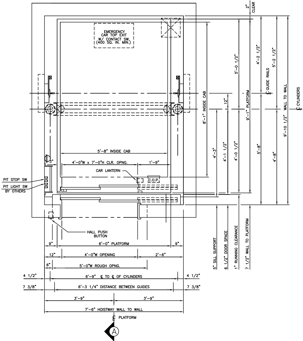
HOISTWAY PLAN
