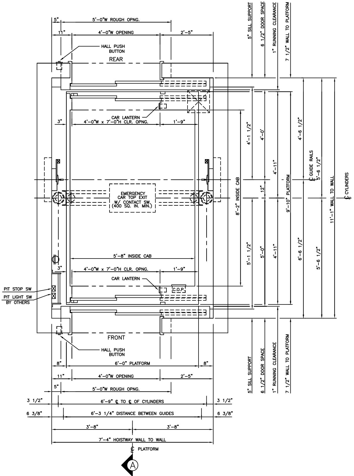
HOISTWAY PLAN
