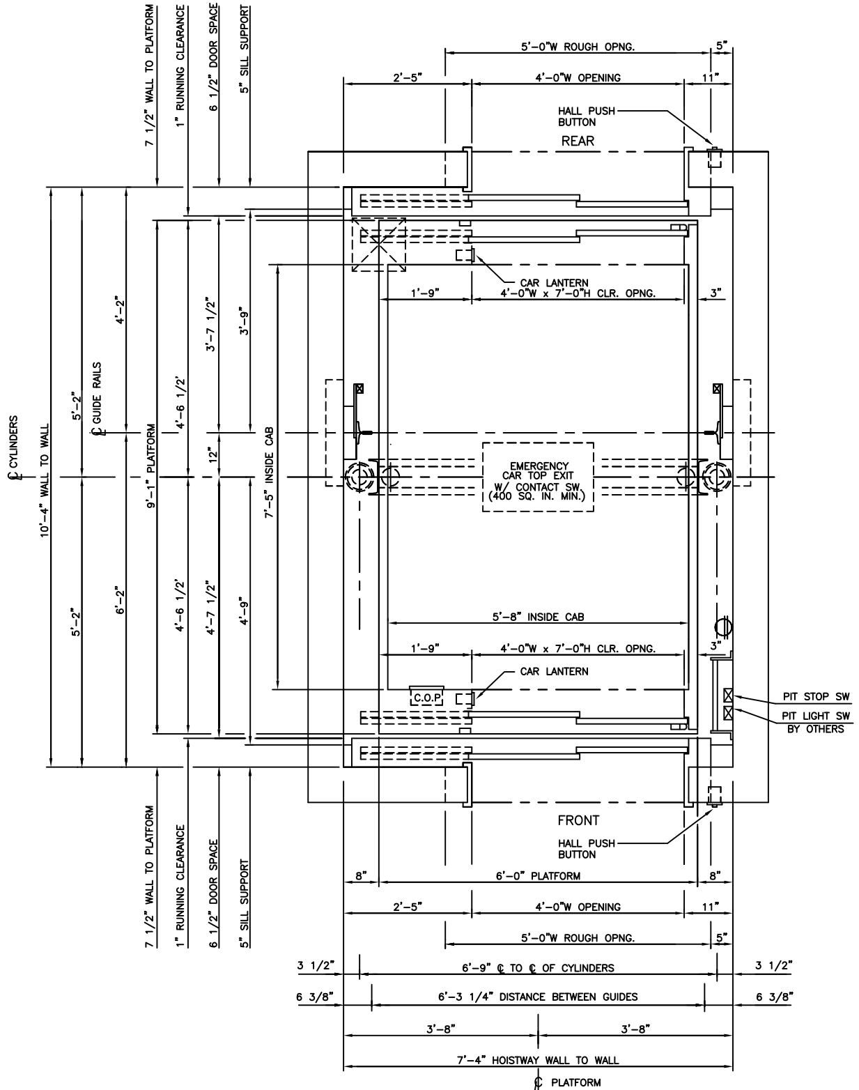
HOISTWAY PLAN
