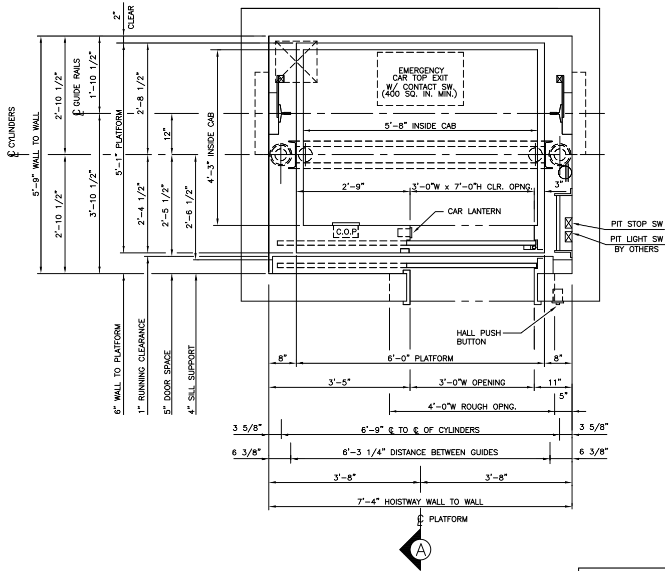
HOISTWAY PLAN
