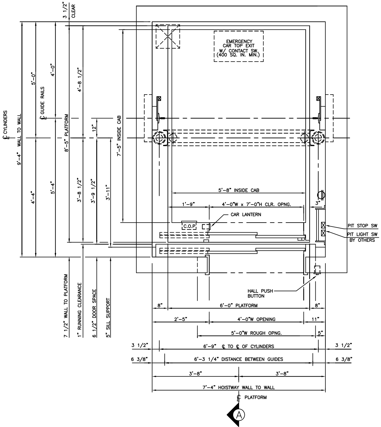
HOISTWAY PLAN
